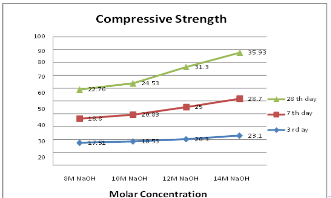
Figure 8: Variation of compressive strength with molar concentration of NaOH
