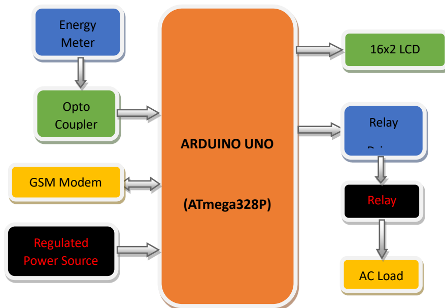
Figure.1 Block Diagram
